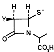
(10) Y = acylamino
